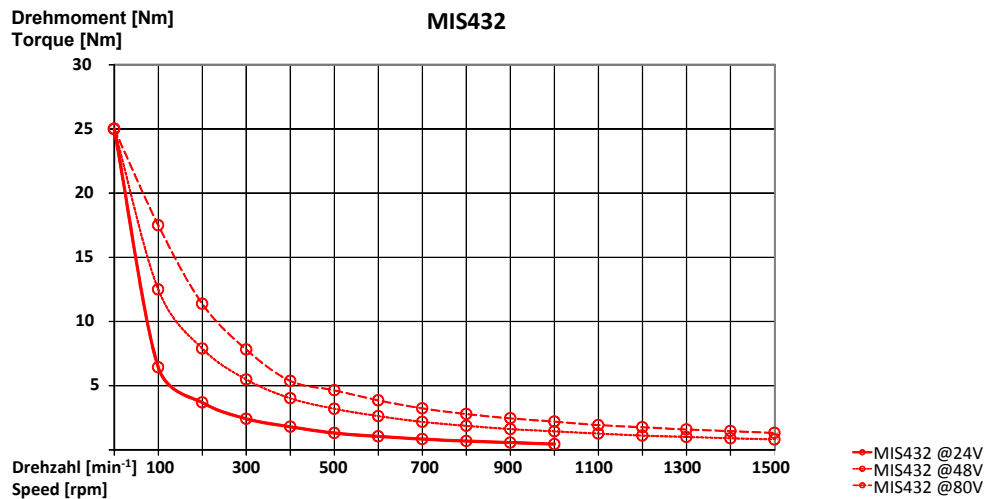
Fig.2: Preliminary Motor characteristic – torque versus speed and supply voltage for MIS432
