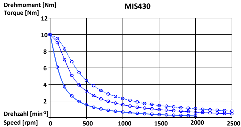
Fig.1: Preliminary Motor characteristic – torque versus speed and supply voltage for MIS430
